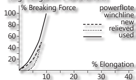
Long-Elongation Characteristics
